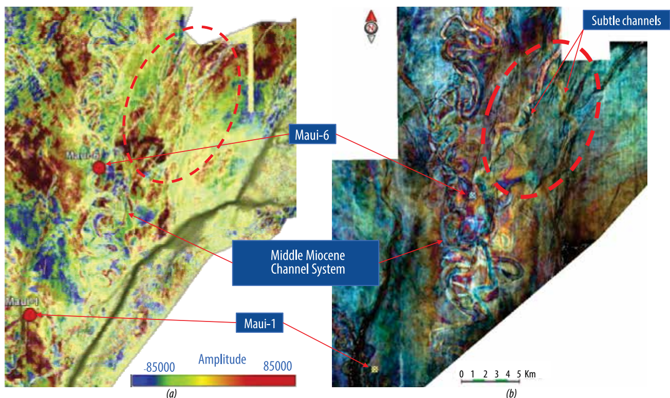
Figure 6. Comparison between (a) horizon from N30-N40 interval using the isoproportional slicing method in Kröeger et al. [17] and (b) horizon 106 from the horizon stack with colour-blended spectral decomposition with three different frequencies (see Figure 2 for a stratigraphic position). Note that on horizon 106 of the horizon stack, the subtle channels in the dash, red circle area, and the overall geometry of the Middle Miocene channel system were revealed more robustly.
