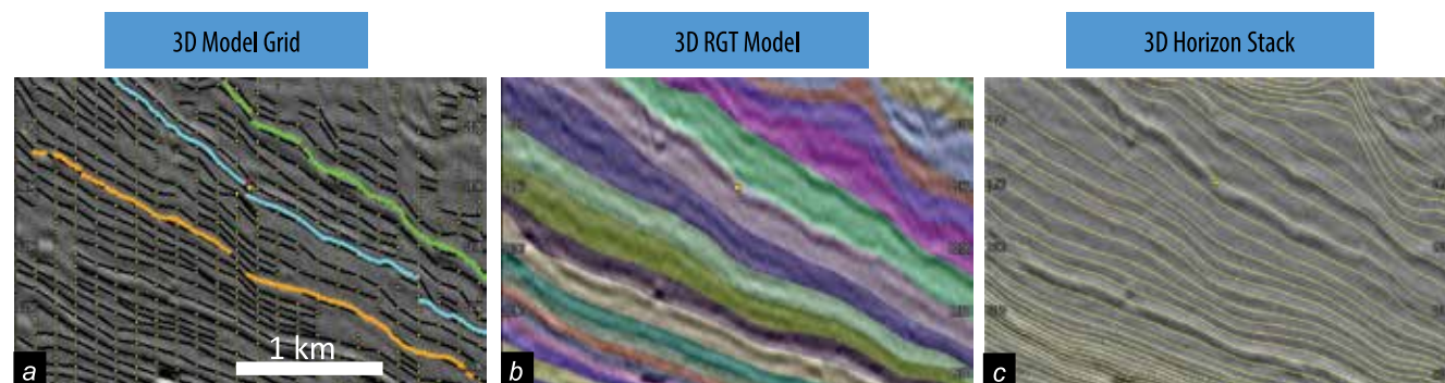
Figure 4. (a) the 3D model grid where key horizon patches can be editable and highlighted in colours, following the interpreter's ideas, (b) 3D RGT model is blended with 3D seismic volume, showing the same geometry. Instead of having seismic amplitudes, there are relative age values assigned to each voxel of the 3D RGT model, (c) The horizon stack comprises dense stratigraphic horizons, representing the geologic time values in the RGT model.
